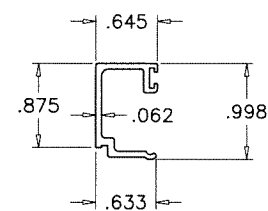
3 GLAZING BEADS
